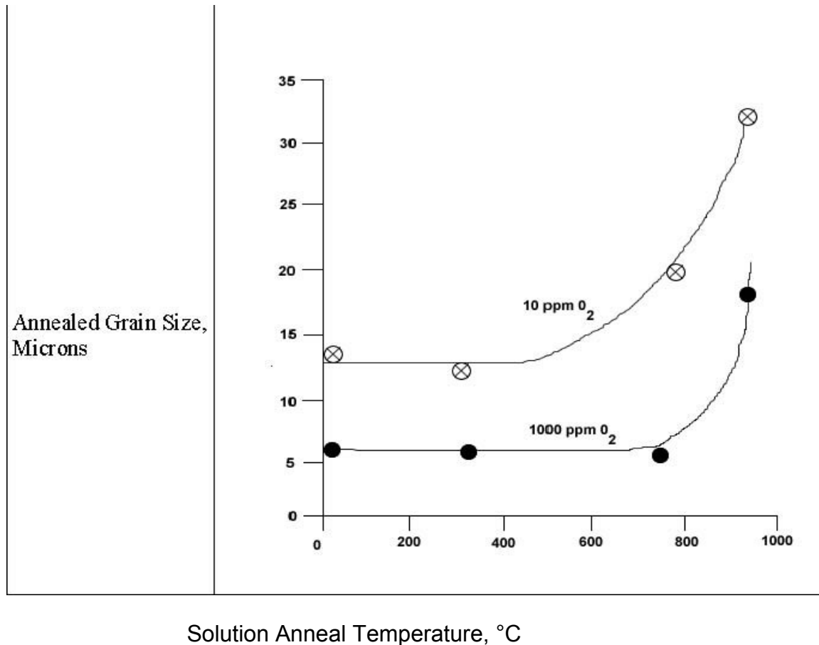
Figure 4- Effect of pre-annealing temperature upon subsequent grain size of annealed ETP copper.
