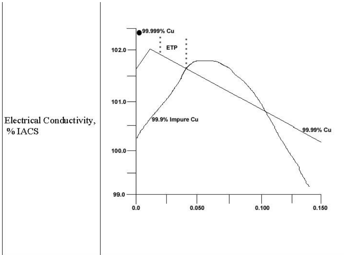
Oxygen Content, Weight% Figure 3- Effect of oxygen content on the electrical conductivity of annealed copper.
